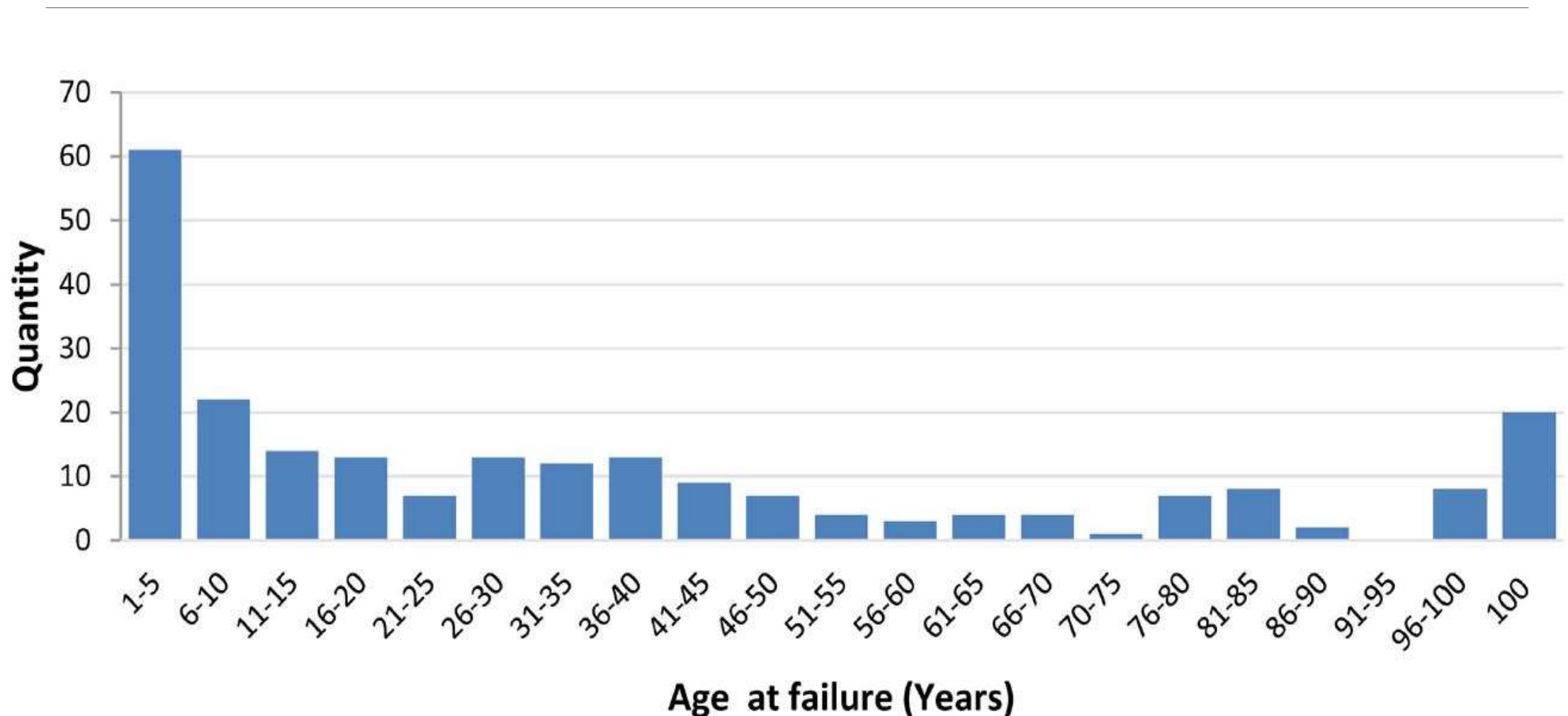
Figure 15. Number of bridges failed at different age groups.
